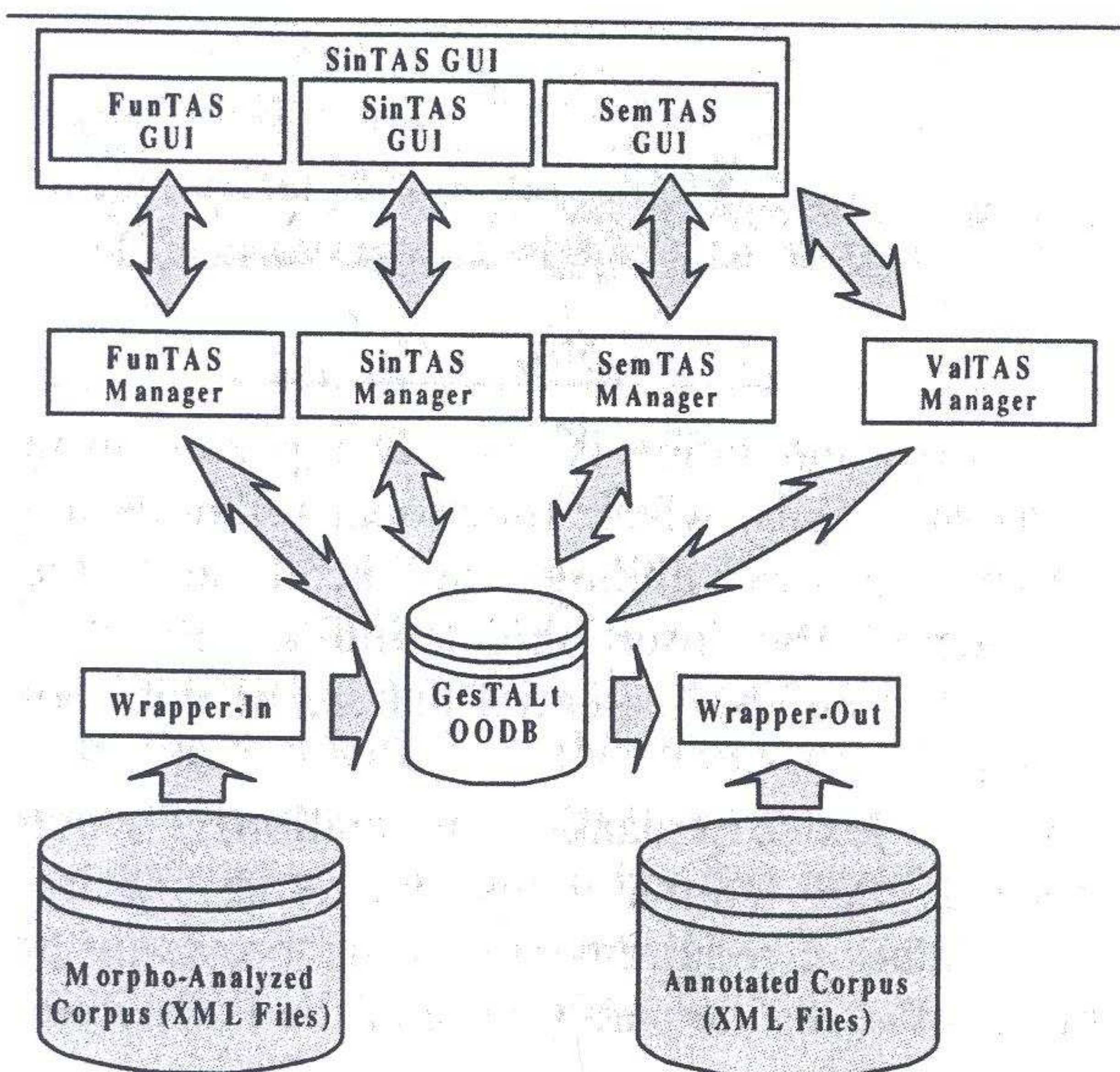
Fig. 3 GestALt architecture
