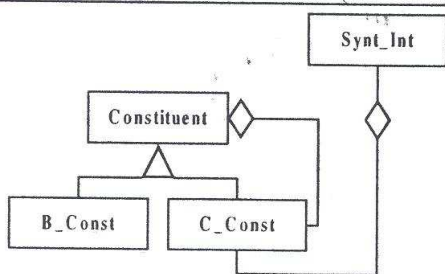
Fig. 1 Syntactic interpretation
