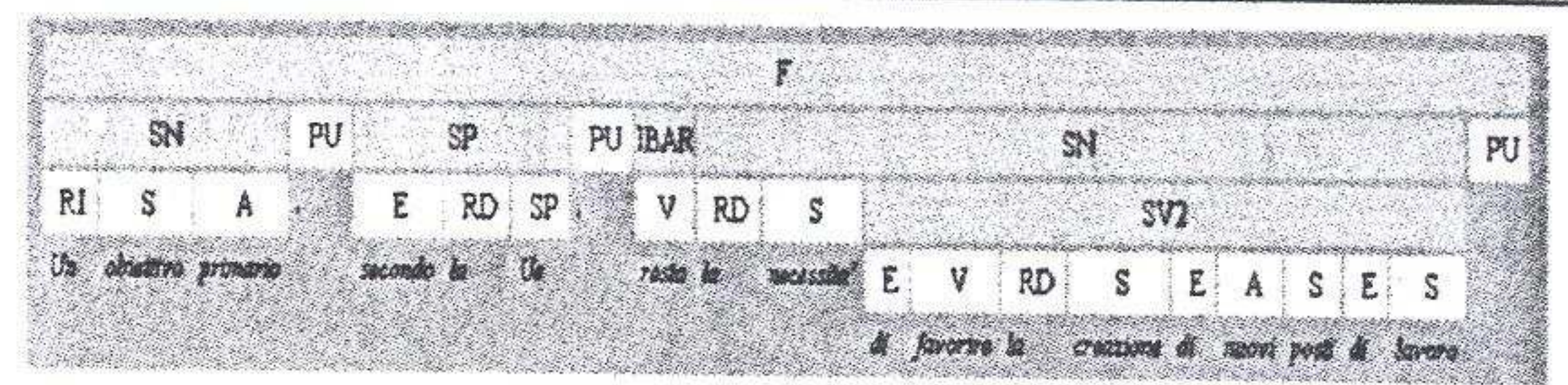
Fig. 2 Strip tree
